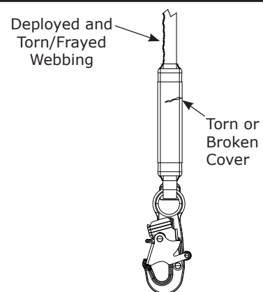
Figure 16 – Load Indicator
