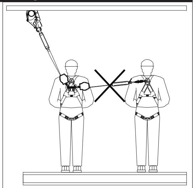
Figure 12 – Incorrect Attachment
