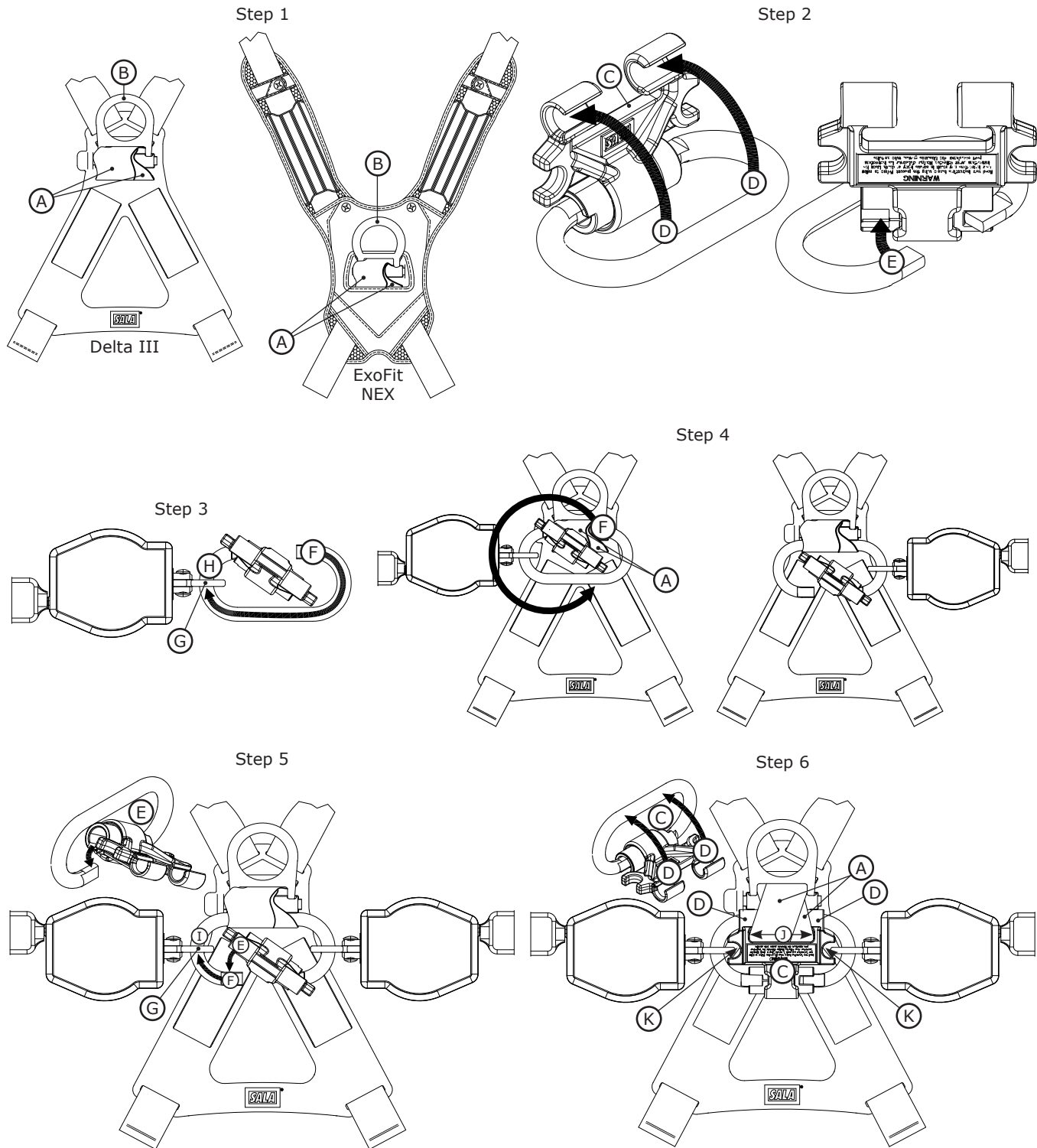
Figure 9 – Twin SRL Harness Interface
