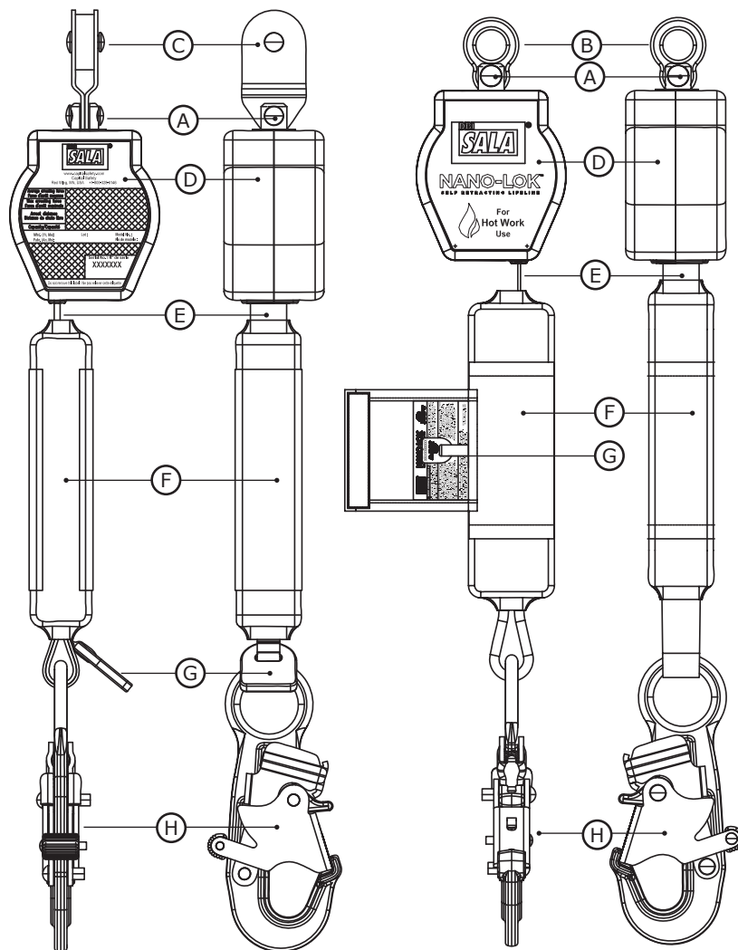
Figure 2 – Nano-Lok Self Retracting Lifeline (SRL) Components
