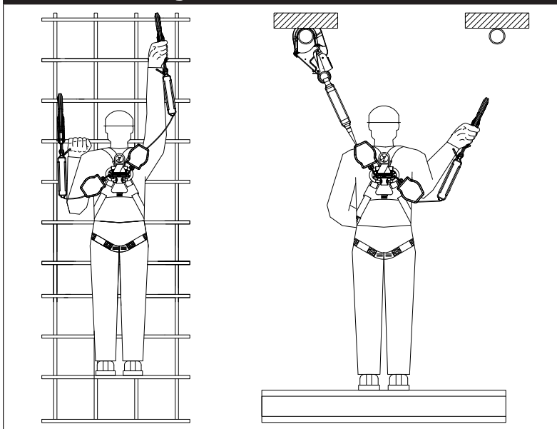
Figure 11 – 100% Tie-Off
