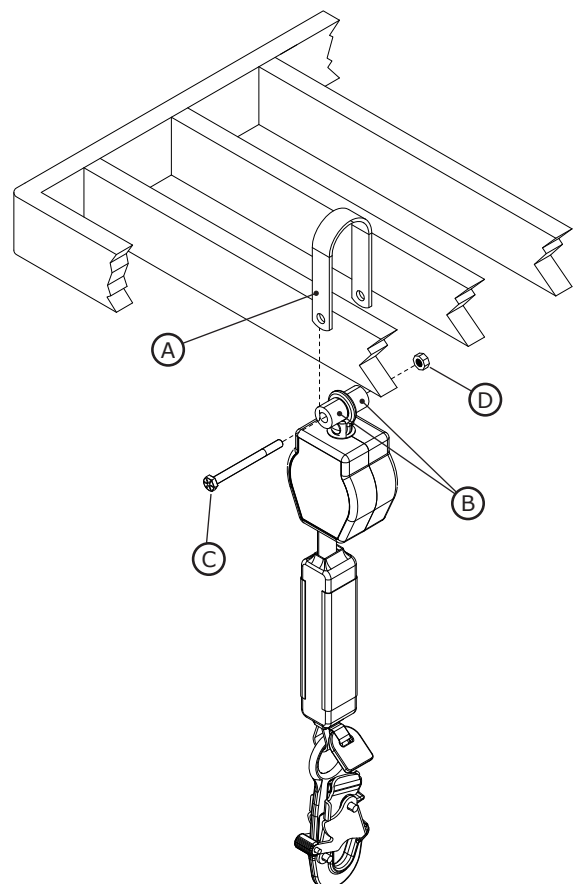
Figure 7 – Cab Mounting
