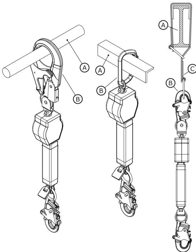
Figure 6 – Anchorage Connections
