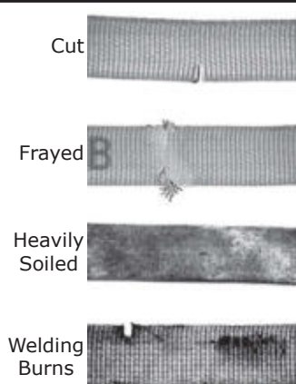
Figure 15 – Web Lifeline
